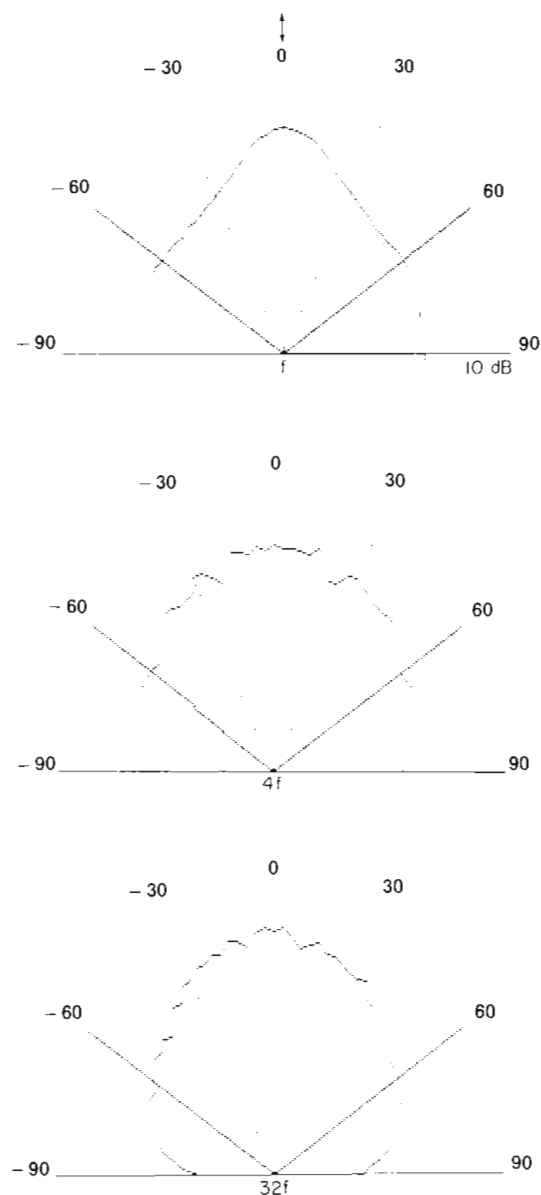
Figure 2. Octave-averaged polar energy response of a QRD surface shows uniform wide-angle diffusion. The polar patterns at f=250\text{Hz} , 4f=1,000\text{Hz} and 32f=8,000\text{Hz} cover five musical octaves. The black trace indicates 0^\circ incidence; the color trace represents 45^\circ .
