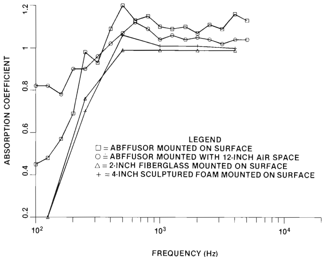
Figure 3. A comparison of absorptive properties of the ABFFUSOR, two inches of fiberglass and four inches of sculptured foam.
