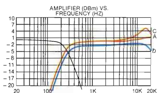
Figure 6. Swept frequency-response curves showing the effects of cable loading on an electronic crossover. The frequency response in curve C shows that ringing outside the audio band does affect what happens inside the audio band.
